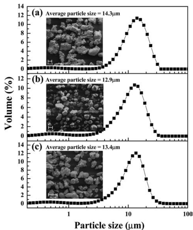
Figure 2. Particle size distribution and SEM micrographs of (a) \text{Ca}_9\text{Y}(\text{PO}_4)_7:0.2\text{Ce}^{3+} , (b) \text{Ca}_9\text{Y}(\text{PO}_4)_7:0.7\text{Gd}^{3+} , and (c) \text{Ca}_9\text{Y}(\text{PO}_4)_7:0.2\text{Pr}^{3+} phosphors.
